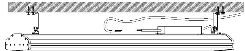
B: Surface Mounting
