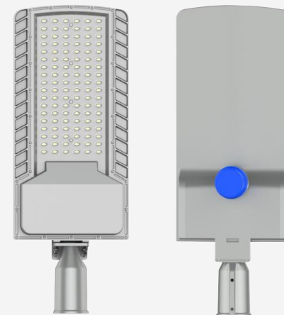
ECO Series LED Street Light S10 PAGE 103-104
