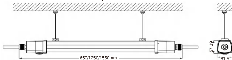
Suspension Mount
